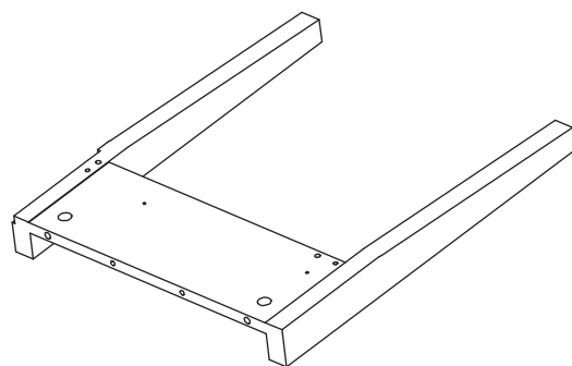
2 Side Panel (Left) Qty 1 (15.55×19.09×1.96")
