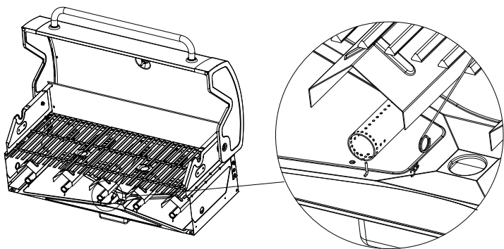
Main Burner Match Lighting
