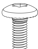
ALLEN KEY SCREW M6*14MM QTY 4 (assembled on stool)
