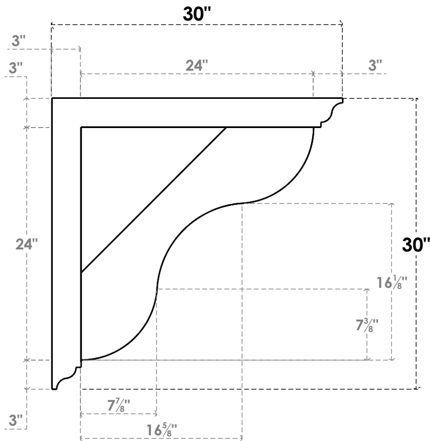
SIDE PROFILE
