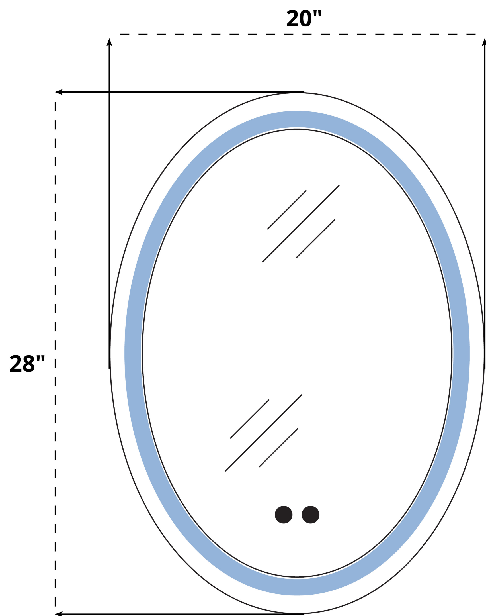
TOP VIEW
