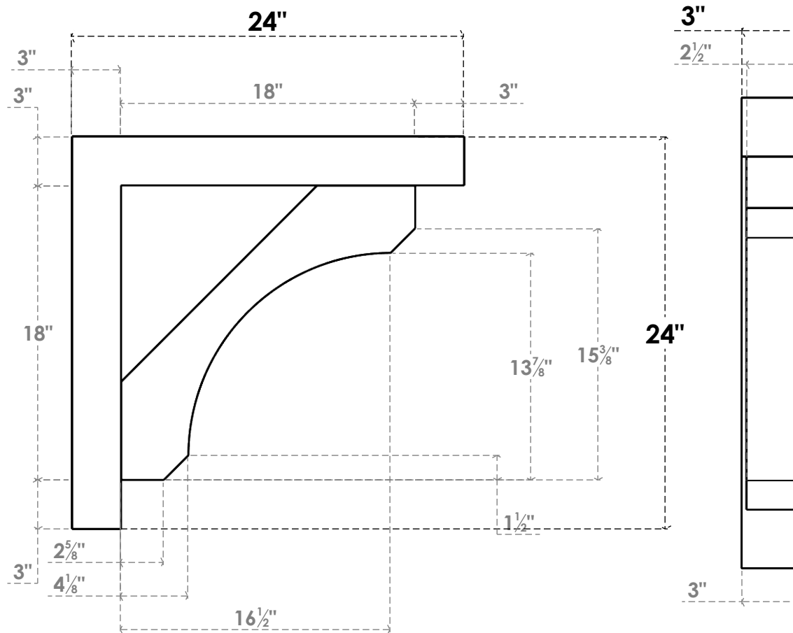
SIDE PROFILE
