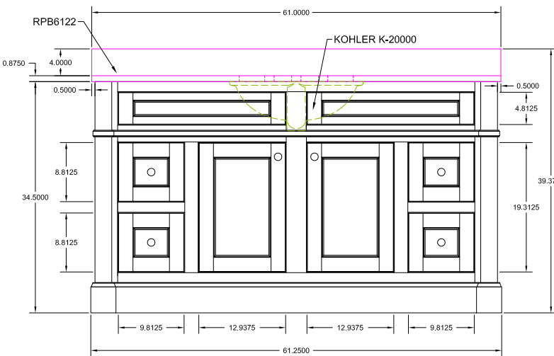
FRONT VIEW
