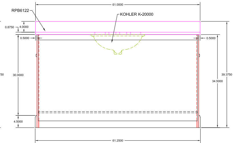
BACK VIEW
