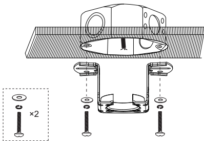
Outlet Box
