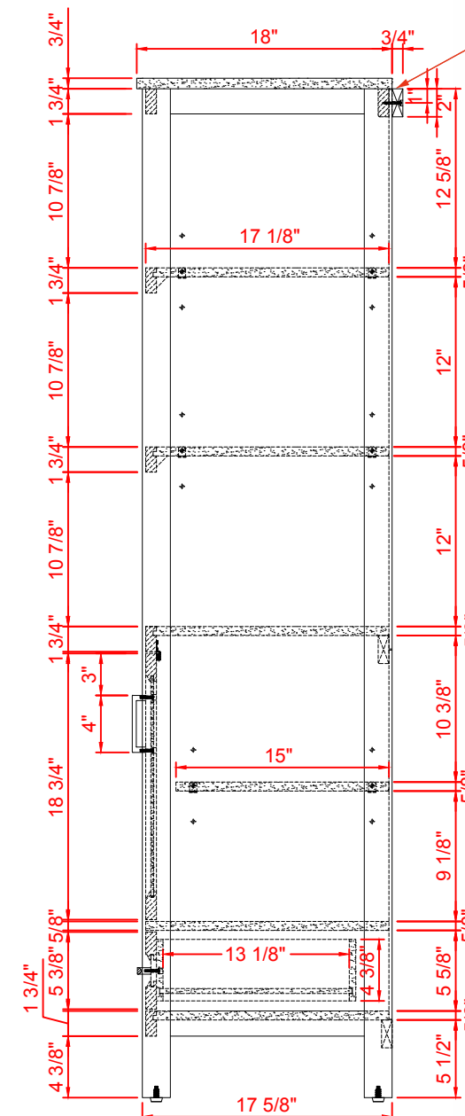
SIDE VIEW
