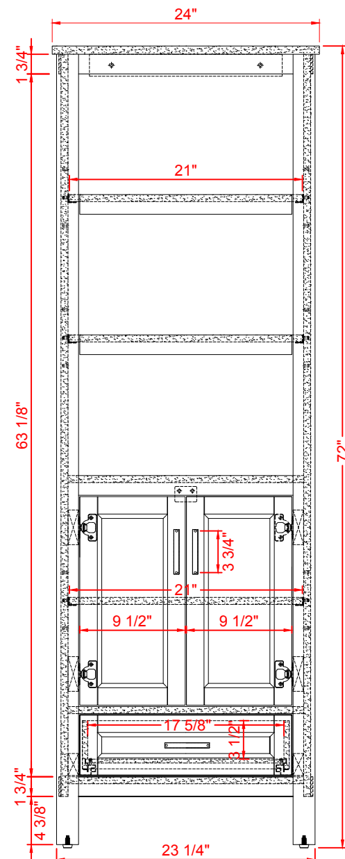
FRONT VIEW
