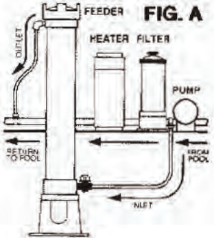
Typical Installation with Heater
