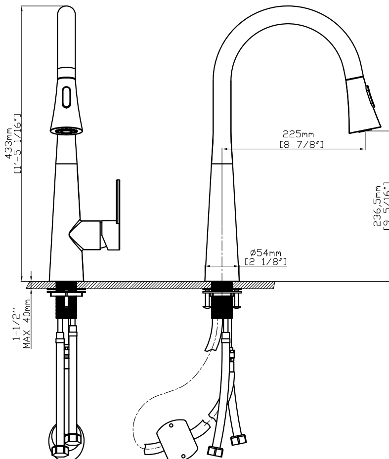
CRITICAL DIMENSIONS
