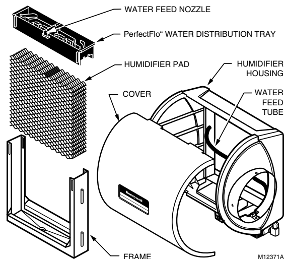
Fig. 1. Humidifier components.
