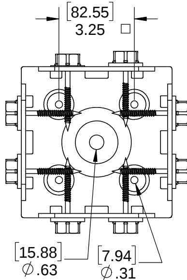
6x6 Post Base Kit (6X6-PB-LS) 56608
