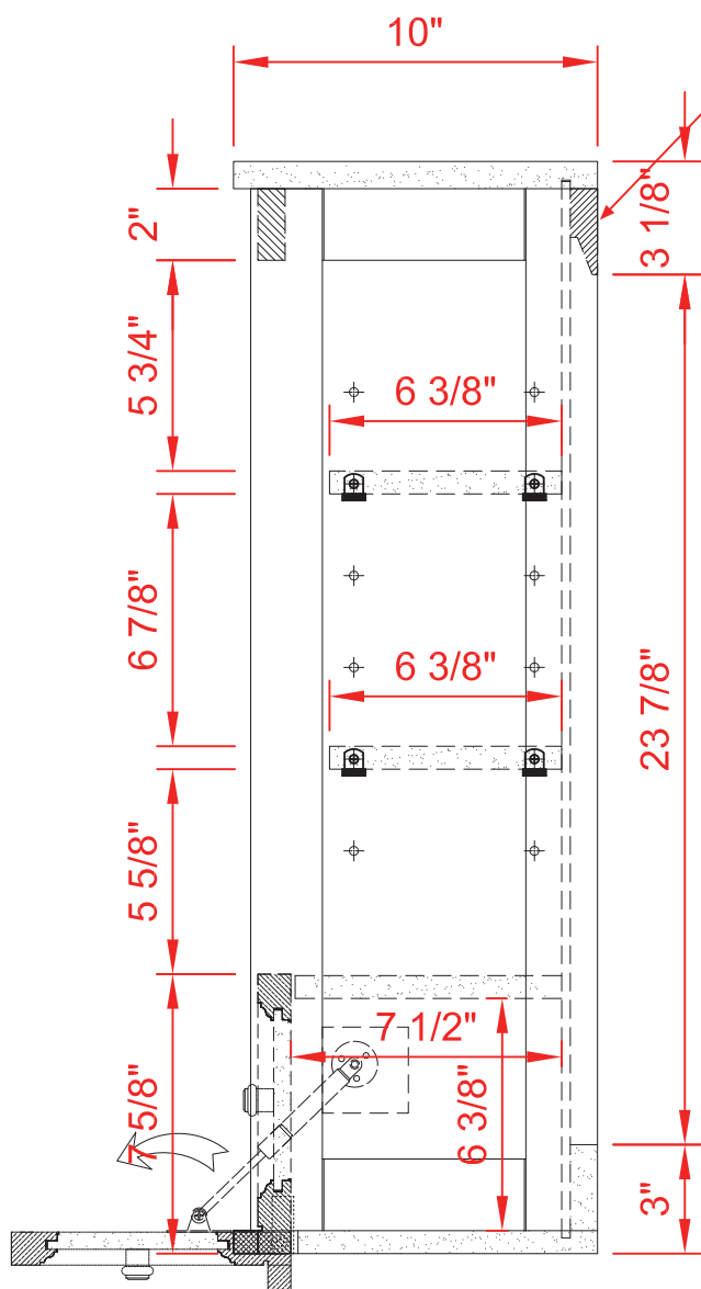
SIDE VIEW
