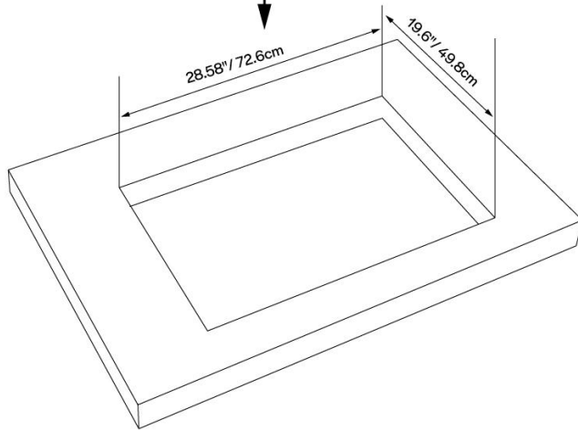
Cutout View
