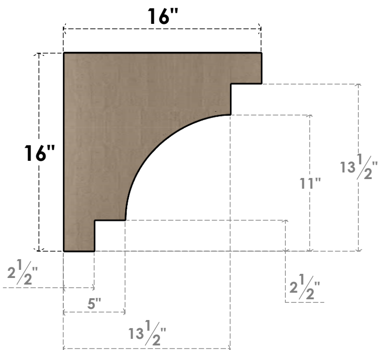
SIDE PROFILE
