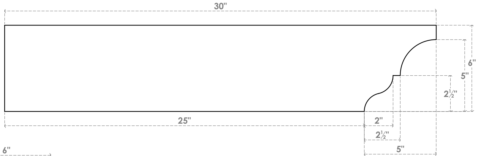
SIDE PROFILE
