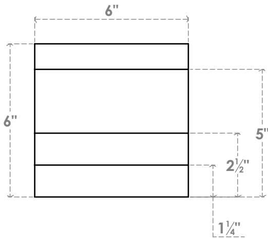
FRONT PROFILE
