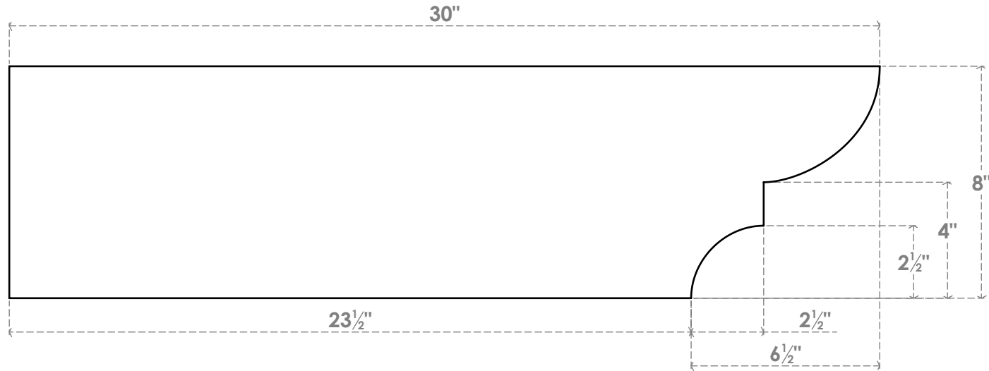
SIDE PROFILE
