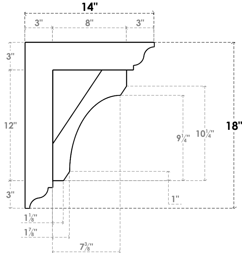
SIDE PROFILE
