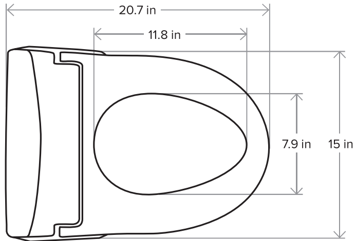
Elongated Top View
