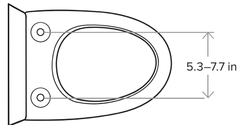
Required Distance Between Mounting Holes
