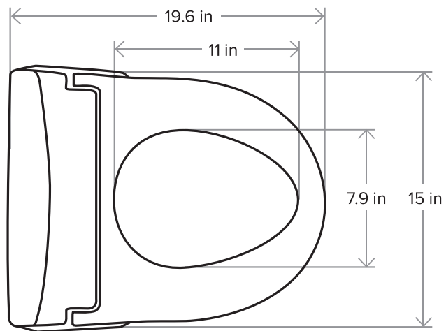
Round Top View
