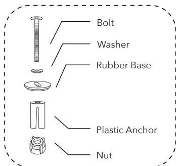
Pre-assembled Fitting
