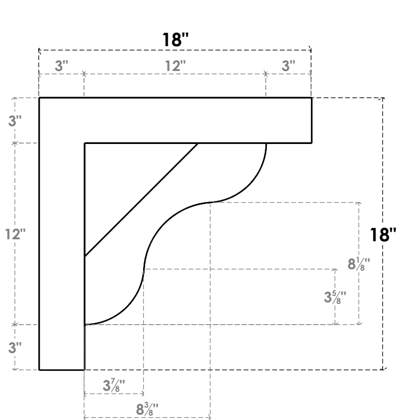
SIDE PROFILE
