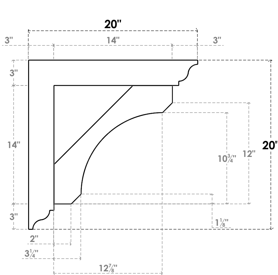
SIDE PROFILE
