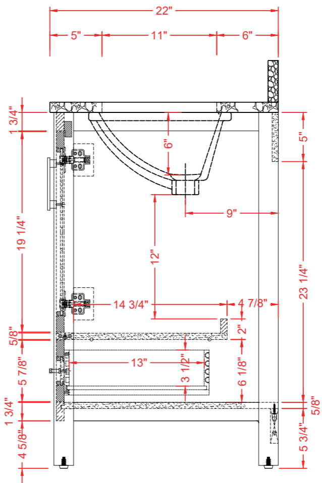
SIDE VIEW
