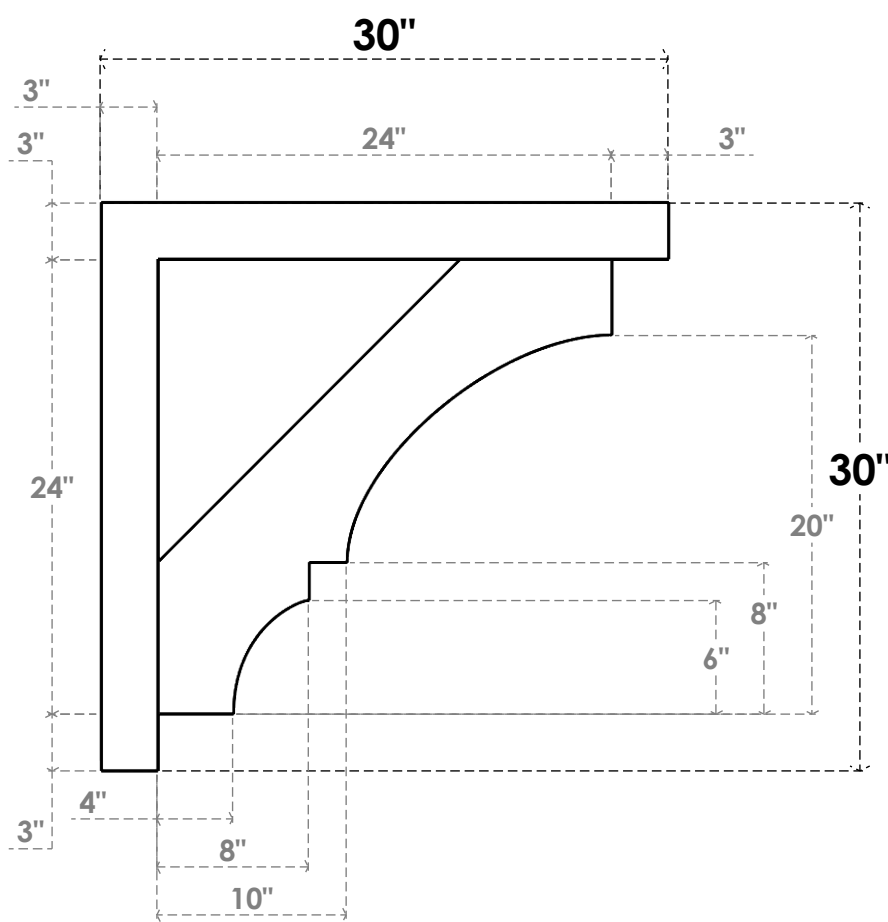
SIDE PROFILE
