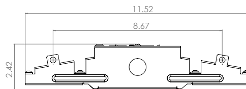
End View: CPHB 12LM, 15LM, 18LM, 24LM, 30LM, ALO13, ALO16, ALO22, ALO34
