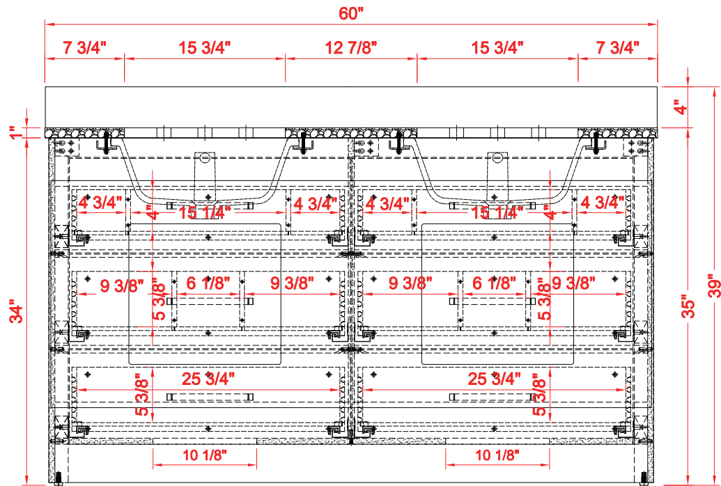
BACK VIEW
