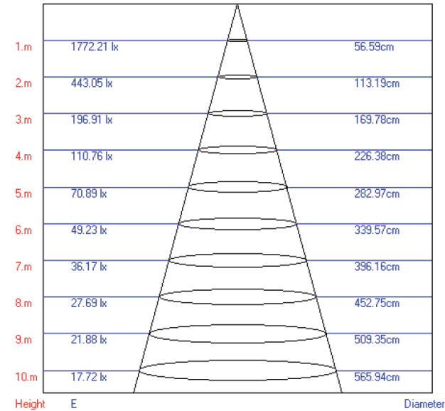
Lux-Distance Curve
