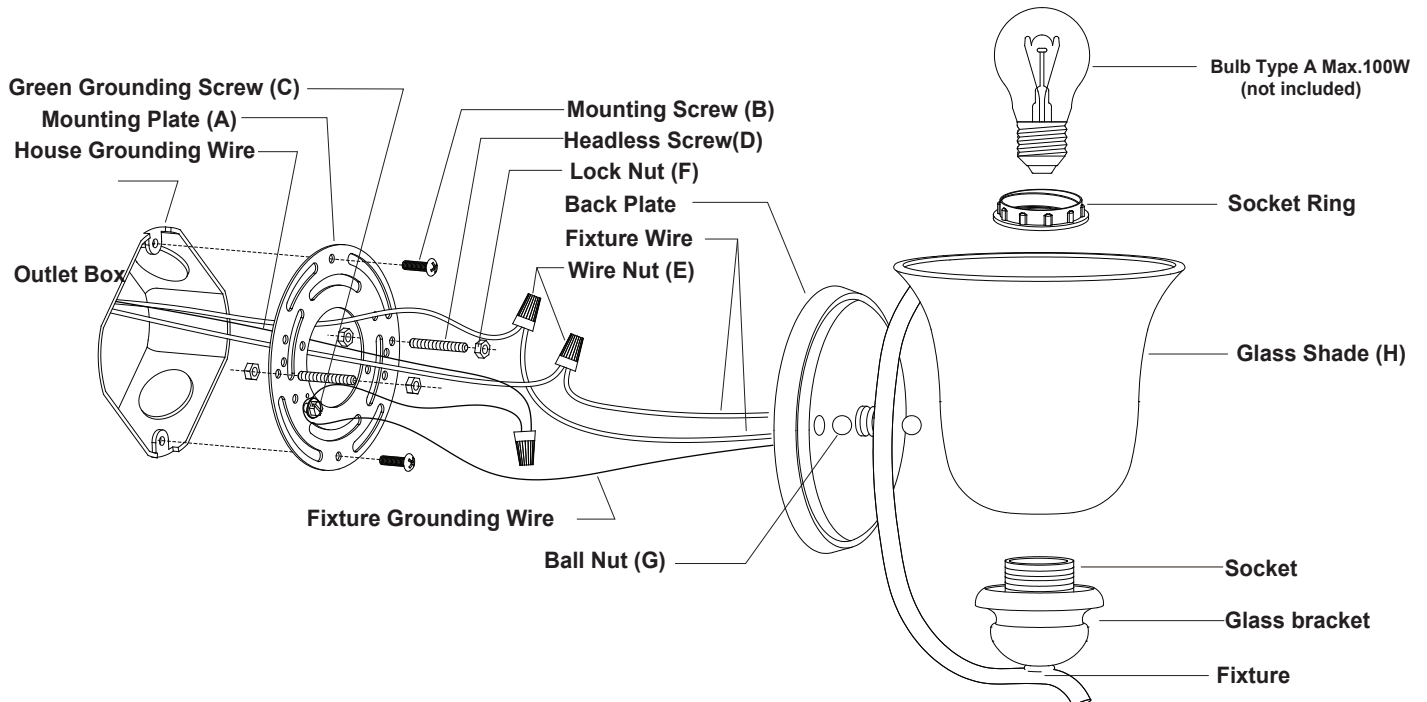
Glass Shade (H) (X1)
