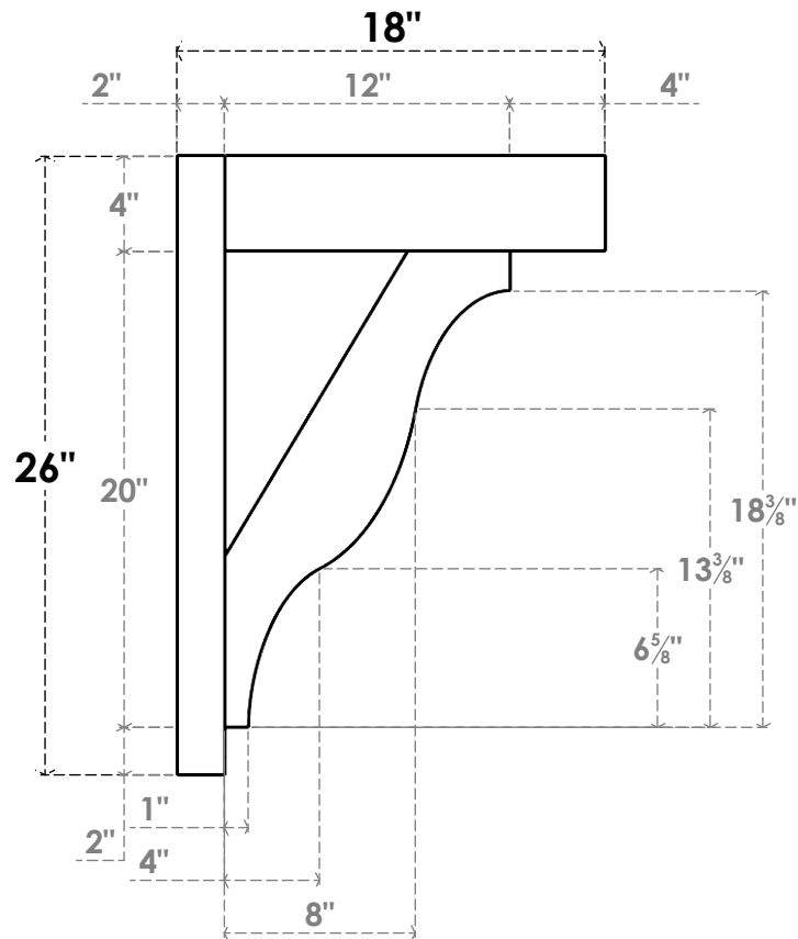
SIDE PROFILE
