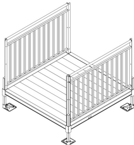
PLATFORM EXTENDER WITH PICKETED GUARDS*
