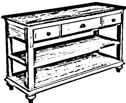
CONSOLE TABLE: 29”H x 18”D x 52.5”W
