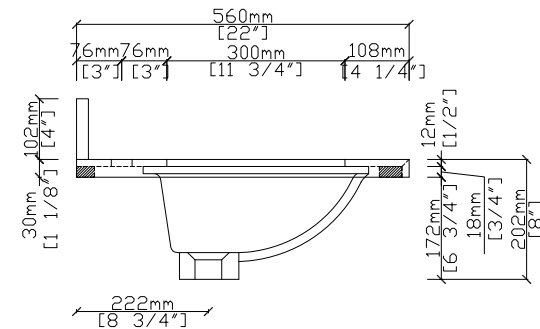
RIGHT VIEW
