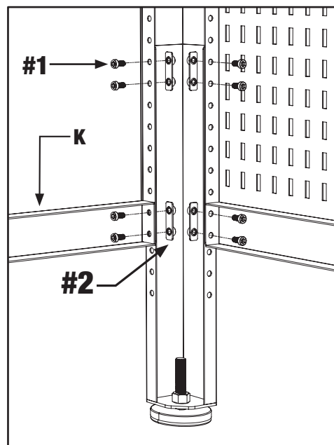
REAR LEG
