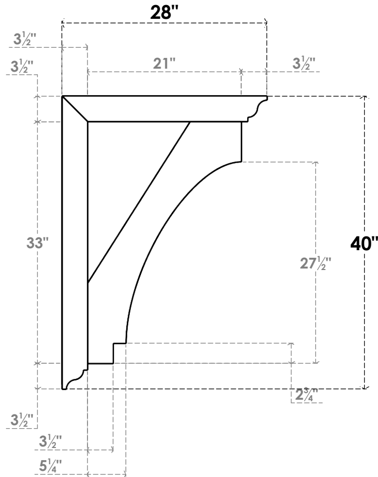
SIDE PROFILE
