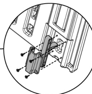
Latch-1 (GS0201018)x1pcs Latch-2 (GS0201019)x1pcs
