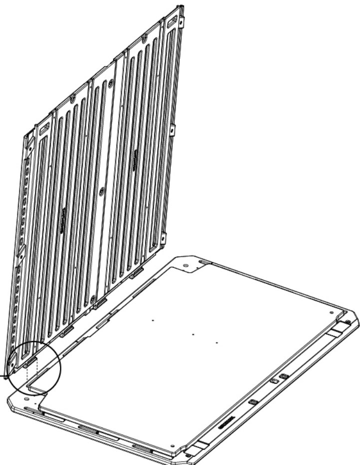
Floor (GS0201001)
