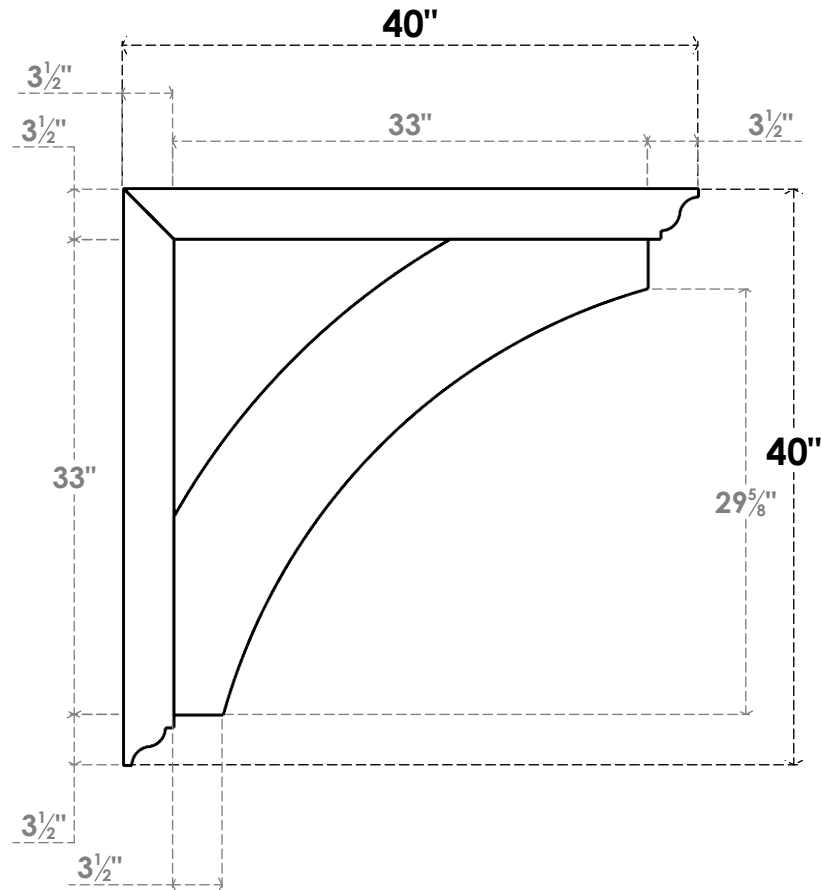
SIDE PROFILE
