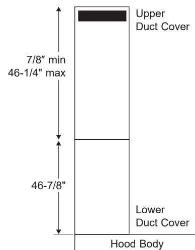
14" High Ceiling Duct Cover Kit
