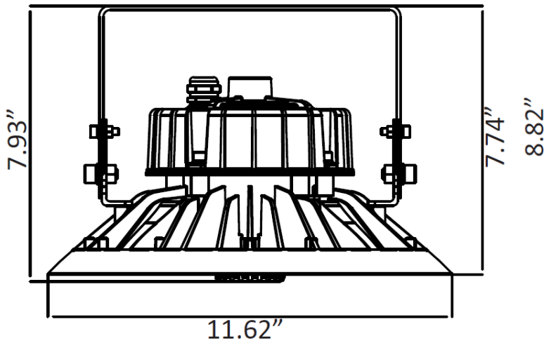
100W – 100W w/ U-Bracket
