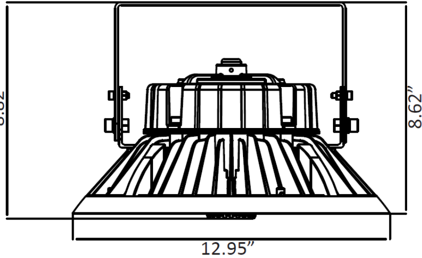
200W – 250W w/ U-Bracket
