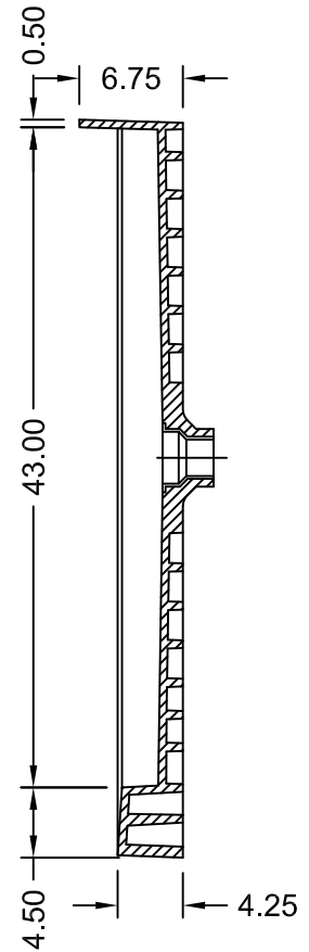
SECTION B-B
