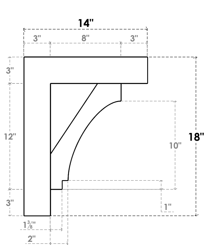
SIDE PROFILE
