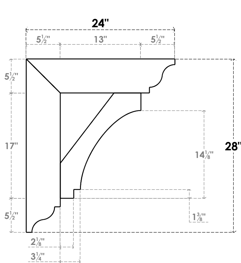
SIDE PROFILE
