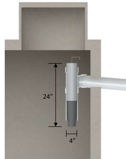
ZOOMED SECTIONED SIDE VIEW
