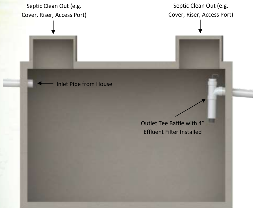
SECTIONED SIDE VIEW OF SEPTIC TANK
