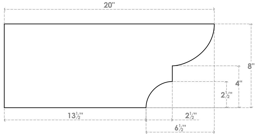
SIDE PROFILE
