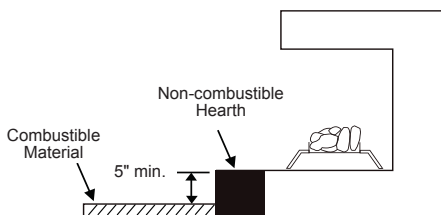
Fig. 9 - Minimum fireplace clearances above combustible flooring
