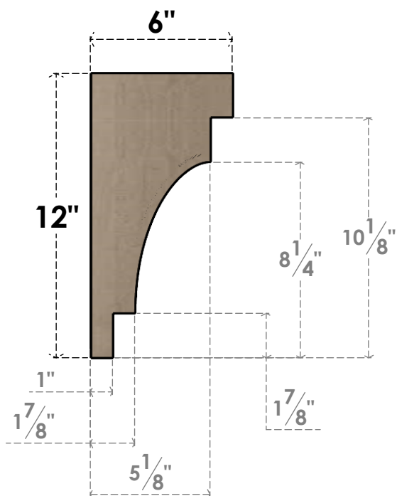
SIDE PROFILE
