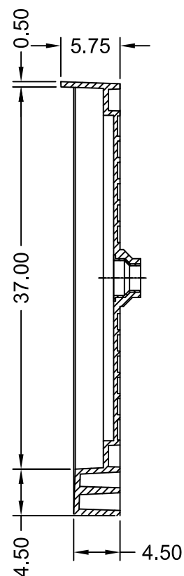
SECTION B-B
