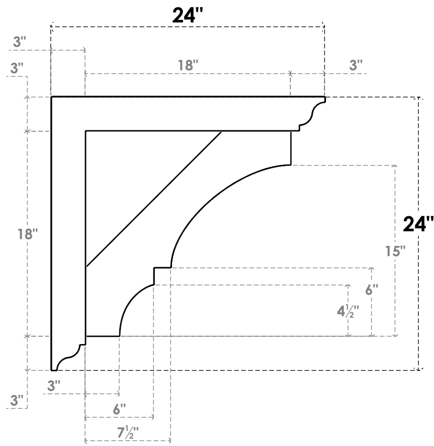
SIDE PROFILE
