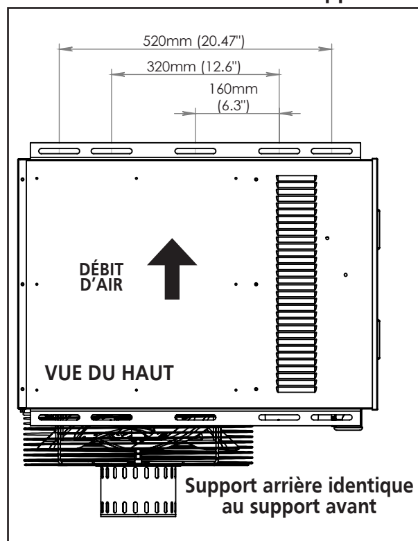
MHU125 Dimensions du Support
