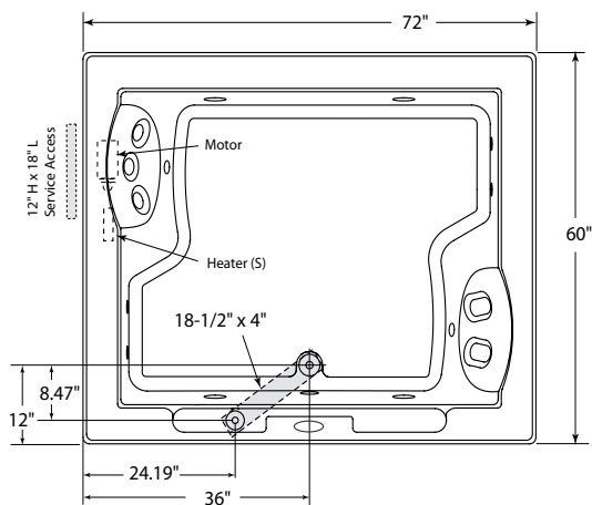
Product Shown: Fuzion™ 7260 Whirlpool Bath Undermount with Illumatherapy Single Right Hand Motor Model: EG25
